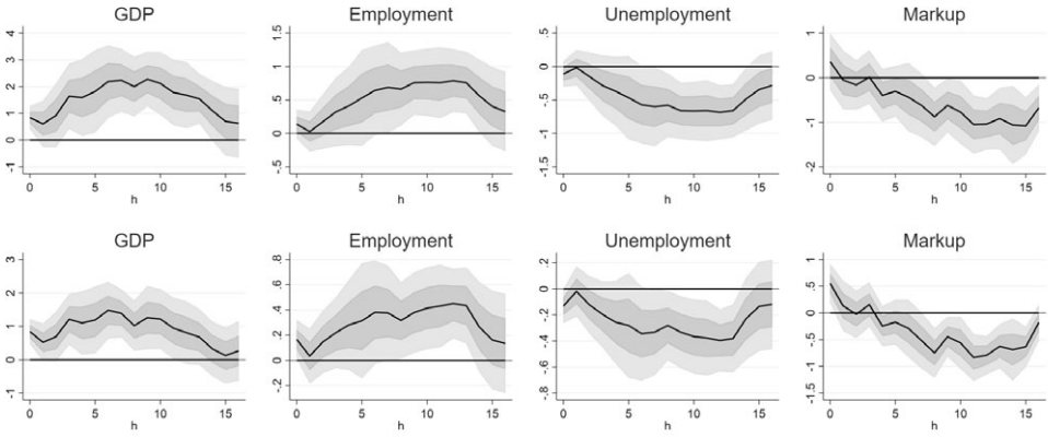
a. Fourth-order time trend specifications
