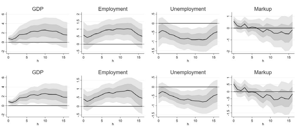
a. Fourth-order time trend specifications
