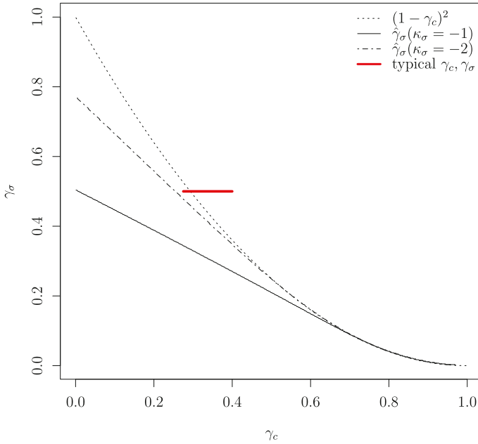
FIGURE B.1. Cutoff \hat{\gamma}_\sigma when \kappa_\sigma = -1 and \kappa_\sigma = -2 .
