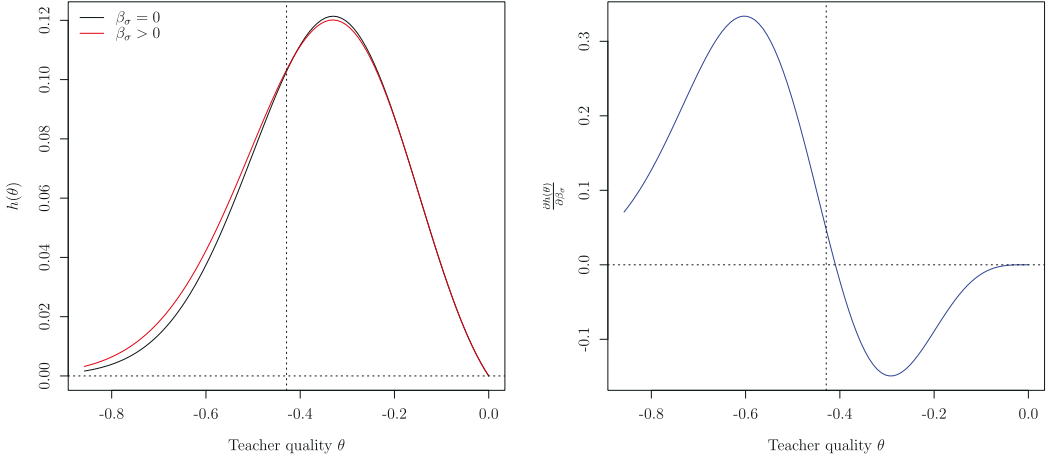
FIGURE B.3. How h(\theta) is affected when \beta_\sigma is increased from zero.
