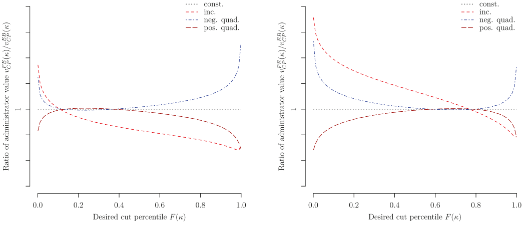
FIGURE B.2. Difference between administrator's value under fixed effects and empirical Bayes, by class size scenario and desired cut point and weight on Type I error, \alpha .
