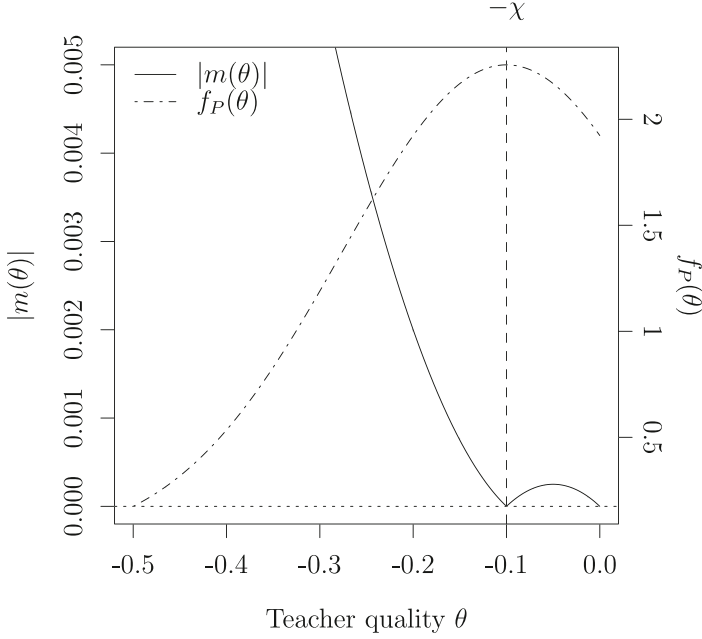
FIGURE C.1. |m(\theta)| and f_P(\theta) .
