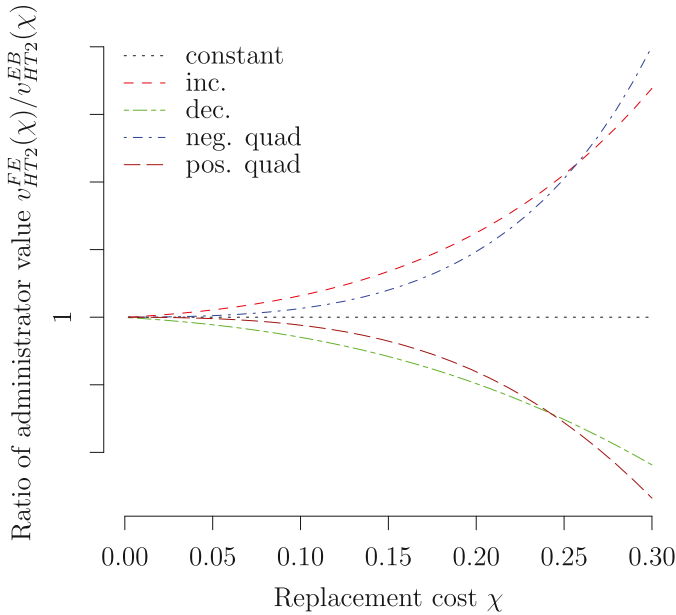
FIGURE C.2. Ratio of values of FE over EB, across class size scenarios.
