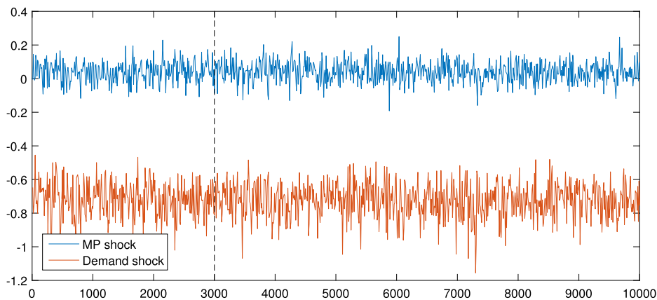
FIGURE C.11. MCMC chains for each log shock standard deviation parameter ( \log \sigma ) in the \rho_{ij} = 0.9 simulations in Section C.1.2. See the caption for Figure C.10.
