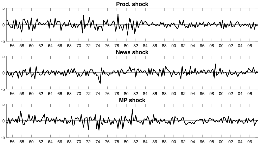
FIGURE C.17. Posterior means of standardized structural shocks ( \varepsilon_{jt}/\sigma_j ) at each point in time, news shock application.
