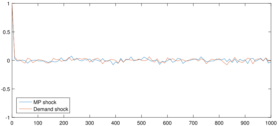
FIGURE C.13. Autocorrelation functions for HMC draws of each log shock standard deviation parameter ( \log \sigma ) in the \rho_{ij} = 0.9 simulations in Section C.1.2. See the caption for Figure C.12.
