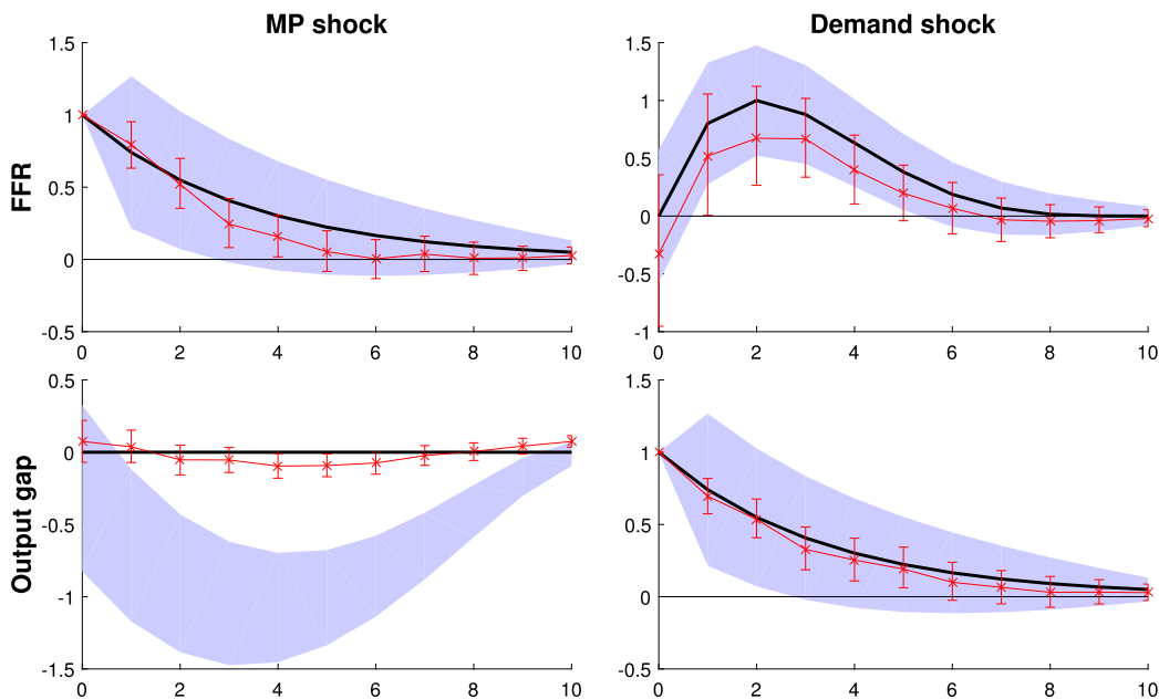
FIGURE C.6. Summary of posterior IRF ( \theta ) draws for the bivariate SVMA model with a prior that misspecifies the cross-correlations between variables. See the caption for Figure C.4.
