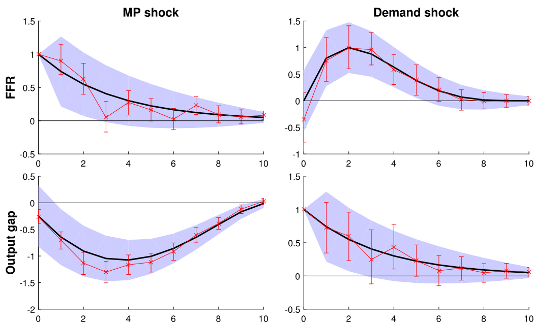
FIGURE C.3. Summary of posterior IRF ( \theta ) draws for the bivariate SVMA model with prior smoothness \rho_{ij} = 0.3 . See the caption for Figure C.1.
