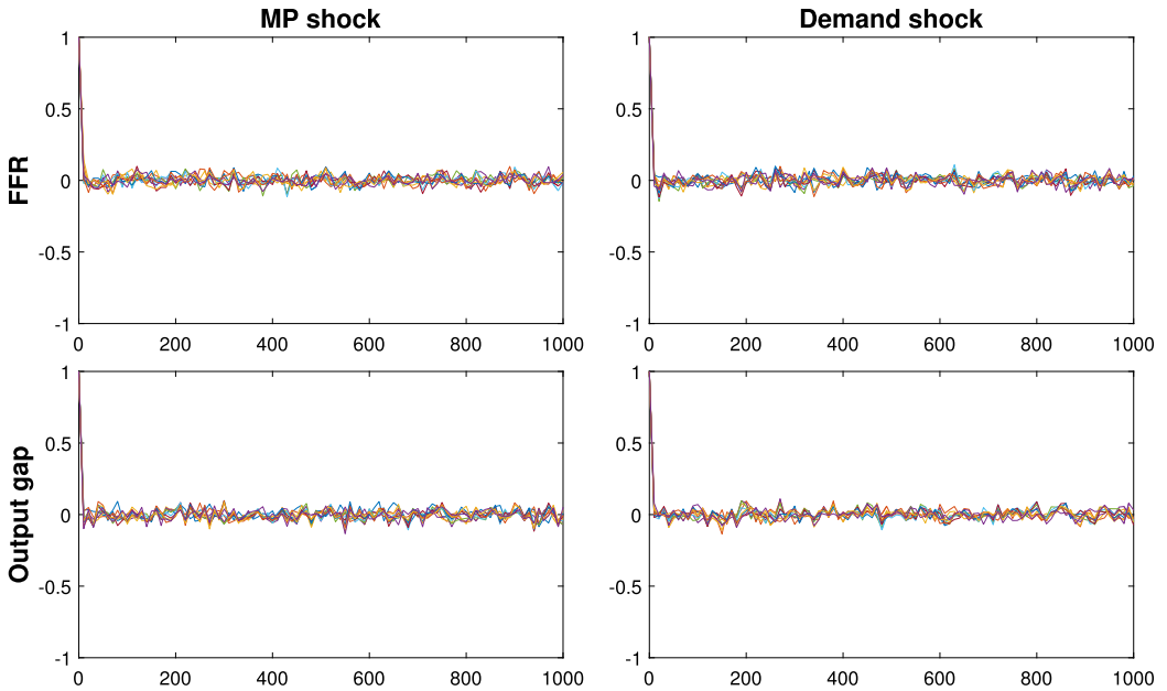
FIGURE C.12. Autocorrelation functions for HMC draws of each IRF parameter ( \theta ) in the \rho_{ij} = 0.9 simulations in Section C.1.2. Each jagged line represents a different impulse response parameter. Only draws after burn-in were used to computed these figures. The autocorrelation lag is shown on the horizontal axes in units of MCMC steps.
