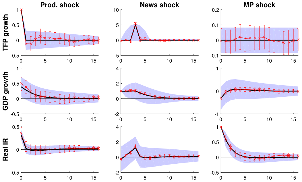
FIGURE C.21. Summary of posterior IRF ( \theta ) draws, simulated news shock data. See the caption for Figure C.1.
