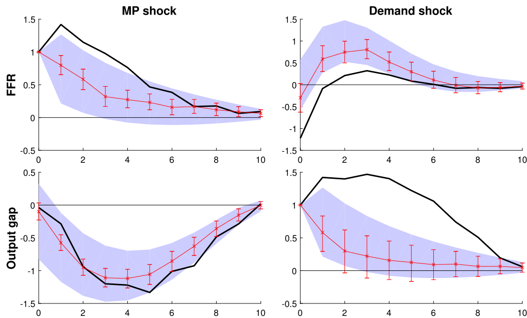
FIGURE C.9. Summary of posterior IRF ( \theta ) draws for the bivariate SVMA model with a grossly misspecified prior whose mode is nevertheless observationally equivalent with the true IRFs. See the caption for Figure C.4.
