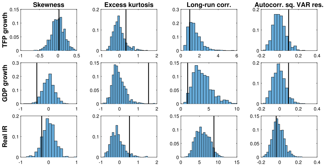
FIGURE C.20. Posterior predictive checks, news shock application. Observed variables along rows, checking functions along columns. Histograms show the distribution of checking function values on simulated data sets based on the posterior parameter draws; thick vertical lines mark checking function values on actual data. Checking functions from left to right: skewness; excess kurtosis; Newey–West long-run variance estimate (20 lags) divided by sample variance; first autocorrelation of squared residuals from a VAR regression of y_t on a constant and 8 lags.
