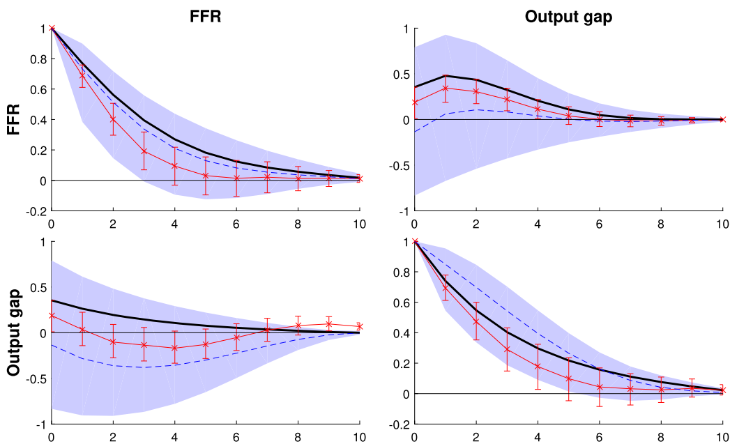
FIGURE C.7. Posterior autocorrelation draws for the bivariate SVMA model with a prior that misspecifies the cross-correlations between variables. See the caption for Figure C.5.
