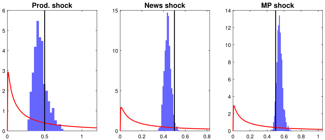
FIGURE C.22. Summary of posterior shock standard deviation ( \sigma ) draws, simulated news shock data. See the caption for Figure C.2.
